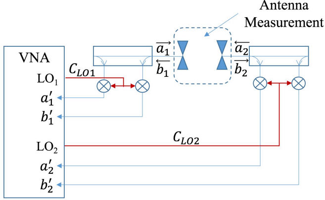
Figure 2. Simplified signal block diagram for a bi-directional frequency-converting two-port VNA measurement. The source is not shown as changes in the source signal are minimized by the ratioed nature of the S-parameter measurement.
